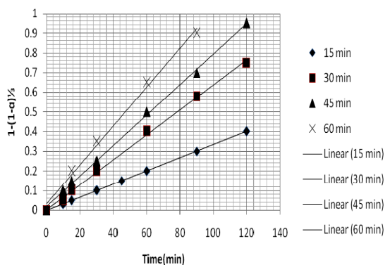
Fig. 7. Linear plots according to the surface reaction model for the effect of grinding time in attritor on leaching rate
